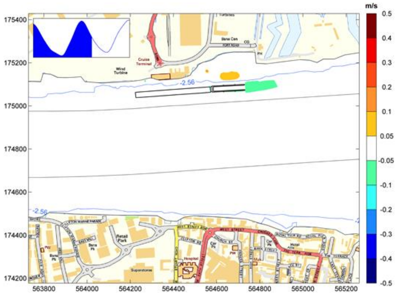
Figure 17.29: Essex Project Site difference in current magnitude at time of peak ebb tide against the baseline model.
